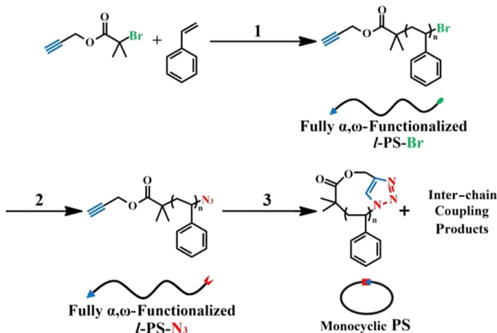
Scheme 1. Synthetic route for cyclic polystyrenes: 1) \text{CuBr} , PMDETA, p -xylene, 85 °C; 2) \text{NaN}_3 , DMF, 24 h, room temperature; 3) \text{CuBr} , PMDETA, 60 °C.
