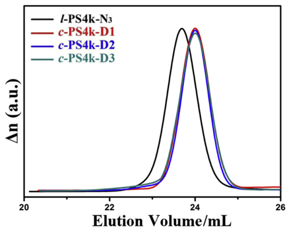
Fig. 4. SEC curves of l -PS4k- N_3 precursor and the corresponding cyclization product in DMF at concentrations of 7.9 \mu\text{mol/L} ( c -PS4k-D1), 15.7 \mu\text{mol/L} ( c -PS4k-D2), and 31.4 \mu\text{mol/L} ( c -PS4k-D3).
