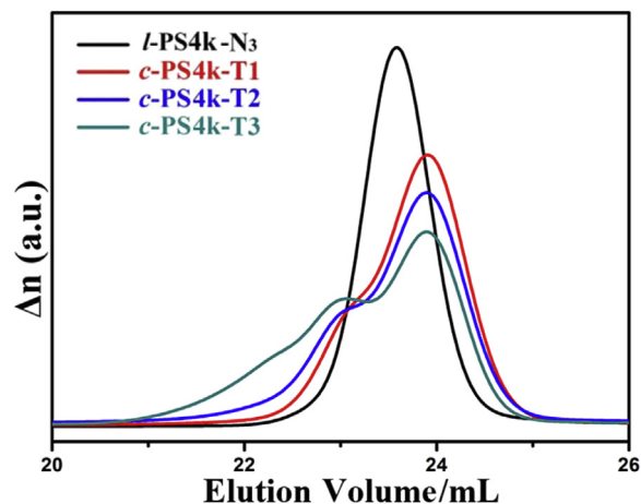
Fig. 5. SEC curves of l -PS4k- N_3 precursor and the corresponding cyclization product in toluene at concentrations of 7.9 \mu\text{mol/L} ( c -PS4k-T1), 15.7 \mu\text{mol/L} ( c -PS4k-T2), and 31.4 \mu\text{mol/L} ( c -PS4k-T3).
